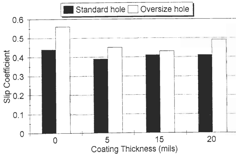
Figure 6. Slip Coefficient vs. Galvanized Coating Thickness
