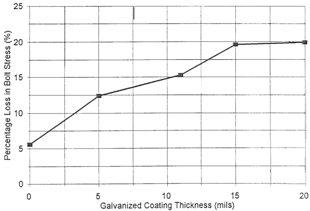
Figure 8. Stress Losses vs. Galvanizing Thickness
