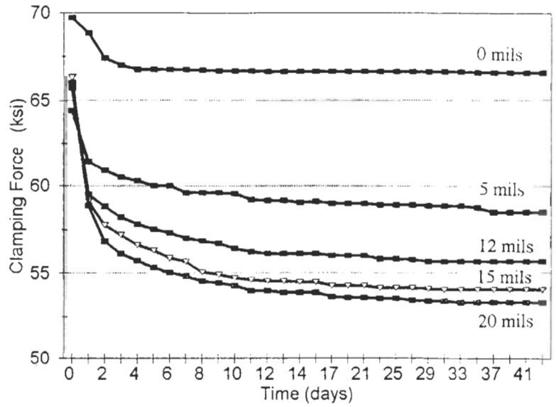
Figure 7. Typical Stress Relaxation Curves
