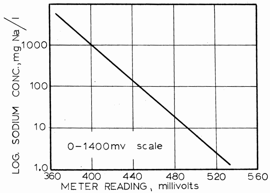
FIG. 4. Sodium Electrode Calibration Curve
