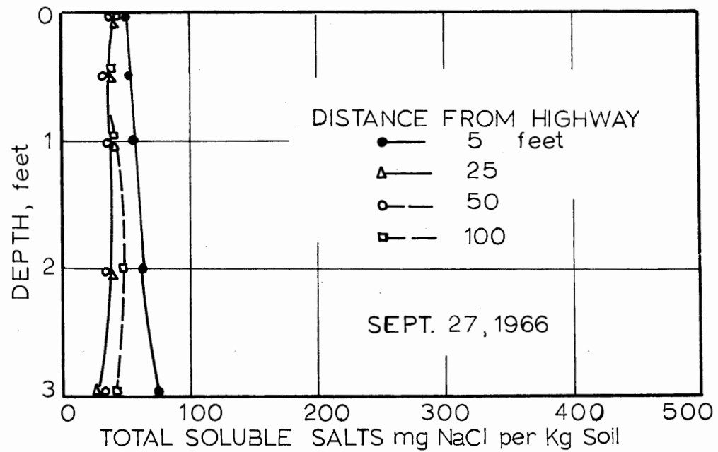
FIG. 8. Depth Profile of Total Soluble Salt Concentration
