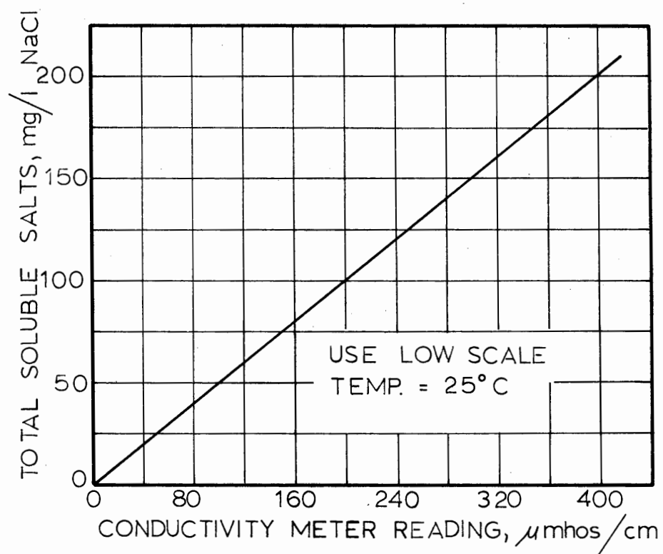
FIG 3 Conductivity Meter Calibration Curve
